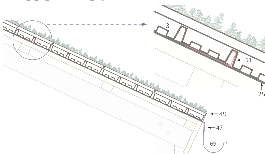
BGreen_it_60_Sedumbakker_Tagfod 10 - 25°
