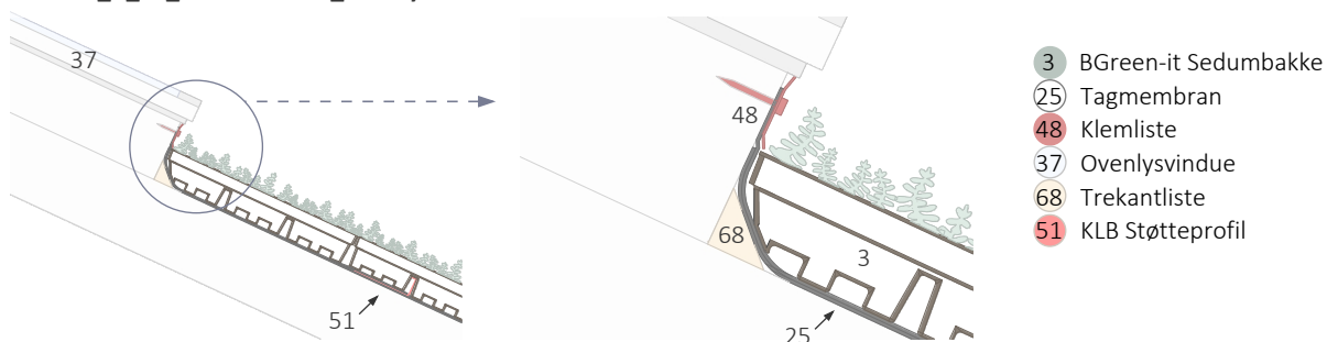
BGreen_it_60_Sedumbakker_Ovenlysvindue
