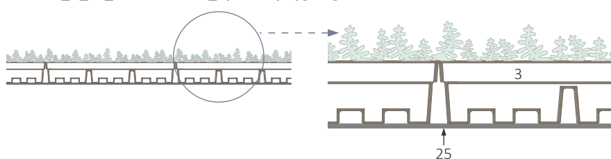
BGreen_it_60_Sedumbakker_Systemopbygning
