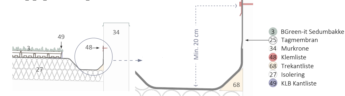
BGreen_it_60_Sedumbakker_Ovenlyskuppel
