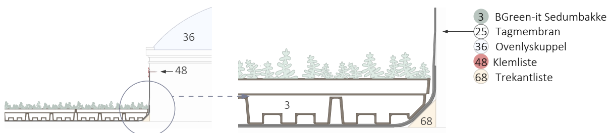
BGreen_it_60_Sedumbakker_Ovenlysvindue
